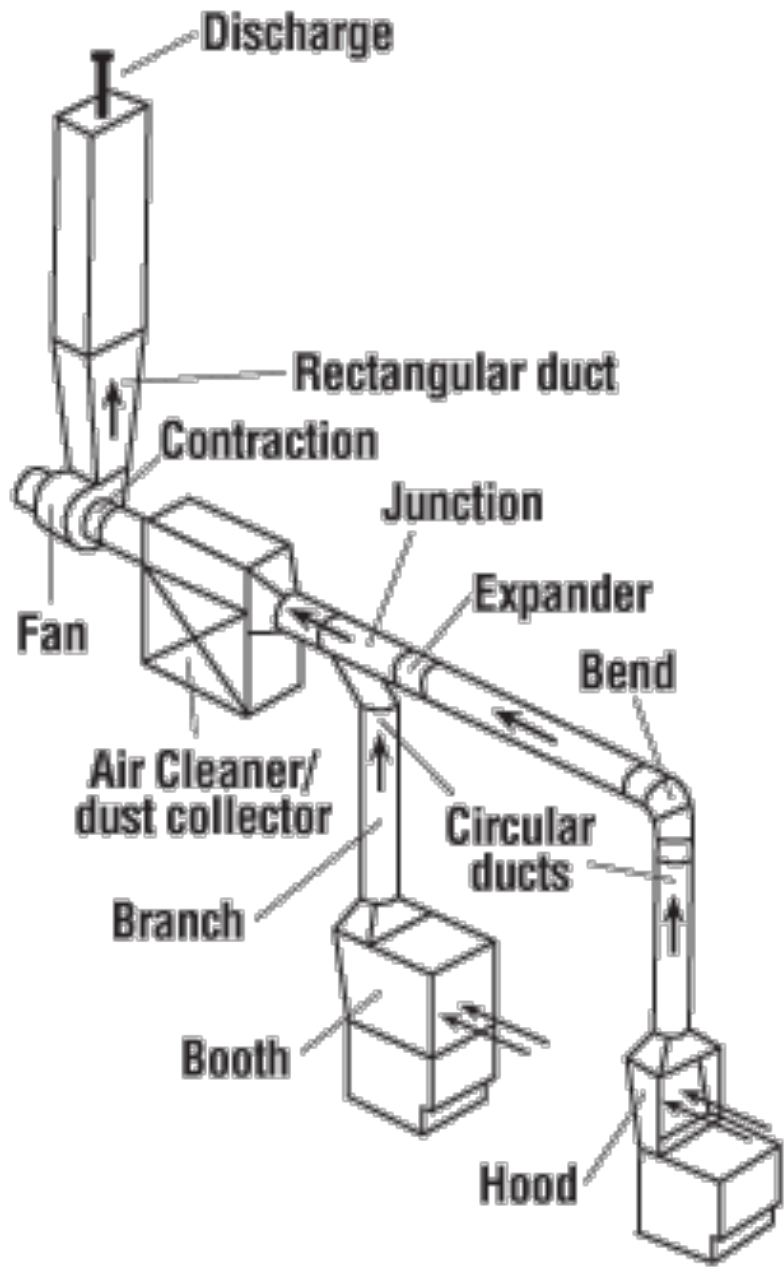
Figure 6 Components of a Local Exhaust Ventilation System
