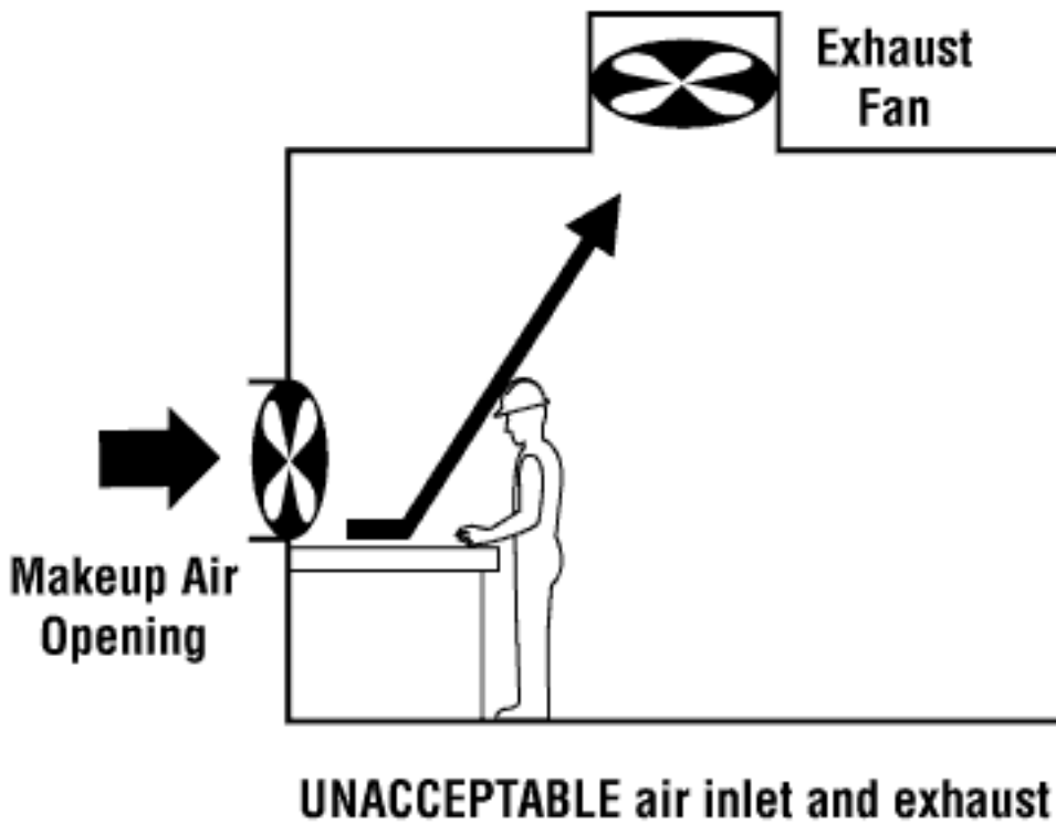
Figure 5 Example of not recommended dilution ventilation layout
