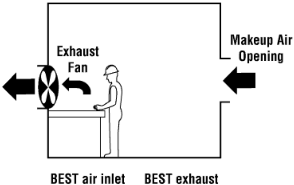
Figure 4 Figures 1 to 4: Examples of recommended dilution ventilation layouts
